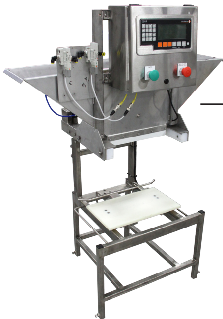
Single Head Drop-Thru 30lb Box Filler with Indexing Conveyor and Incline Exit End for taping boxes at a comfortable height
